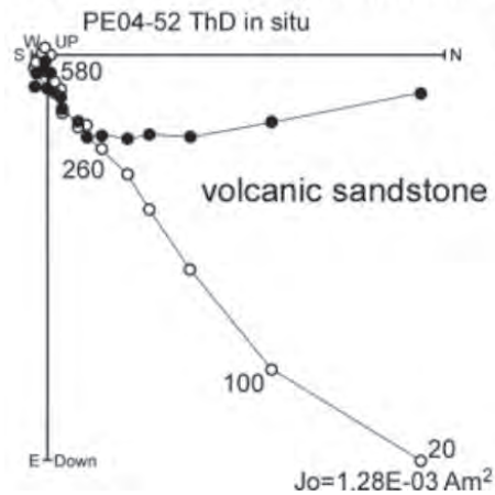
Figure 3. Typical results of progressive thermal demagnetization (PTHD) in in situ coordinates. On the vector-demagnetization diagrams, solid (open) circles are projections of vector end-points on a horizontal (N-S vertical) plane. Numbers are demagnetization levels in °C.
