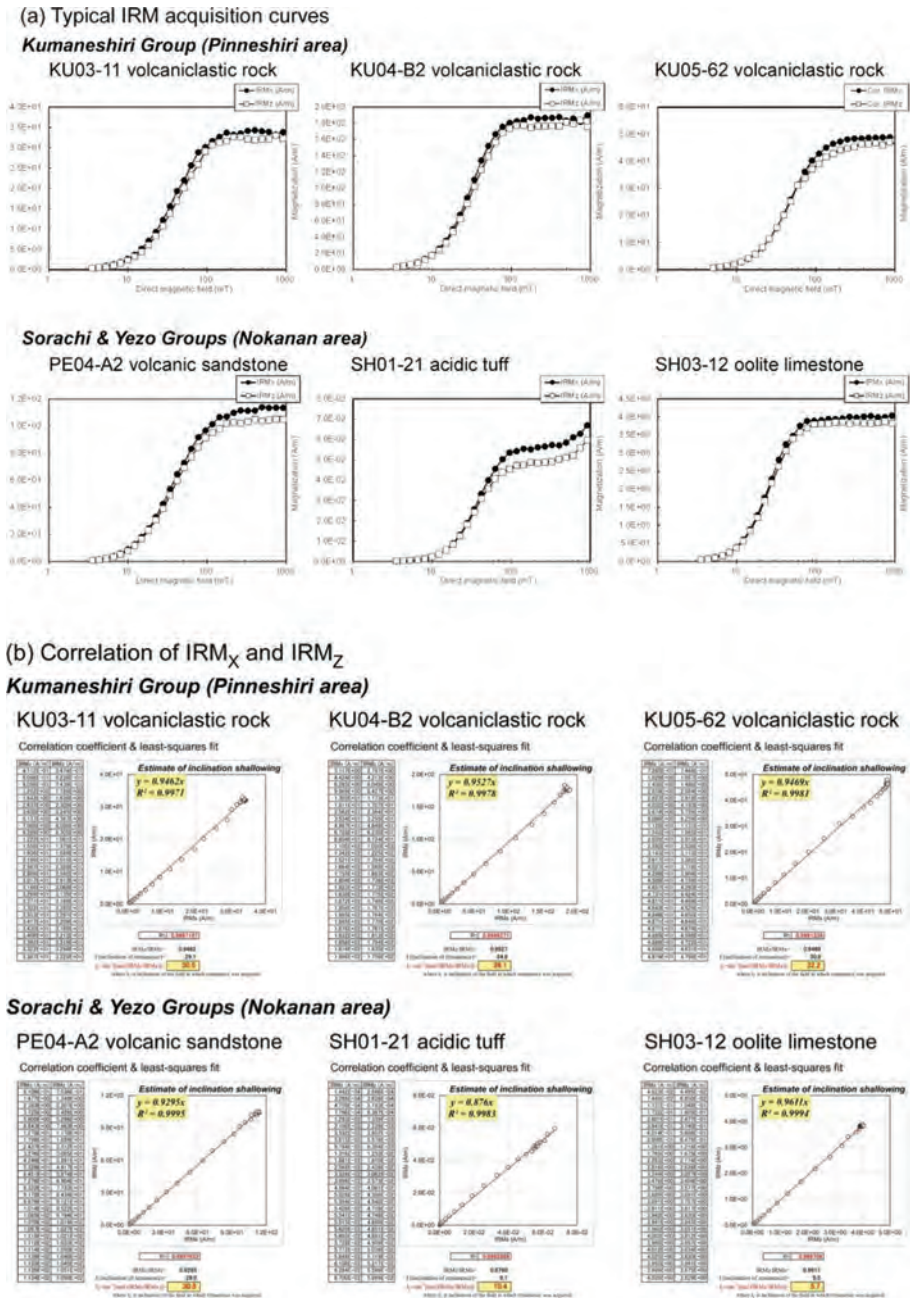
Figure 8. (a) Typical IRM acquisition curves for the bedding-normal (IRM z ) and bedding-parallel components (IRM x ) for selected samples. (b) Gradient of the best-fit correlation line of IRM z versus IRM x used to determine the IRM z /IRM x ratio, which gives an estimate of inclination shallowing in the sediments.
