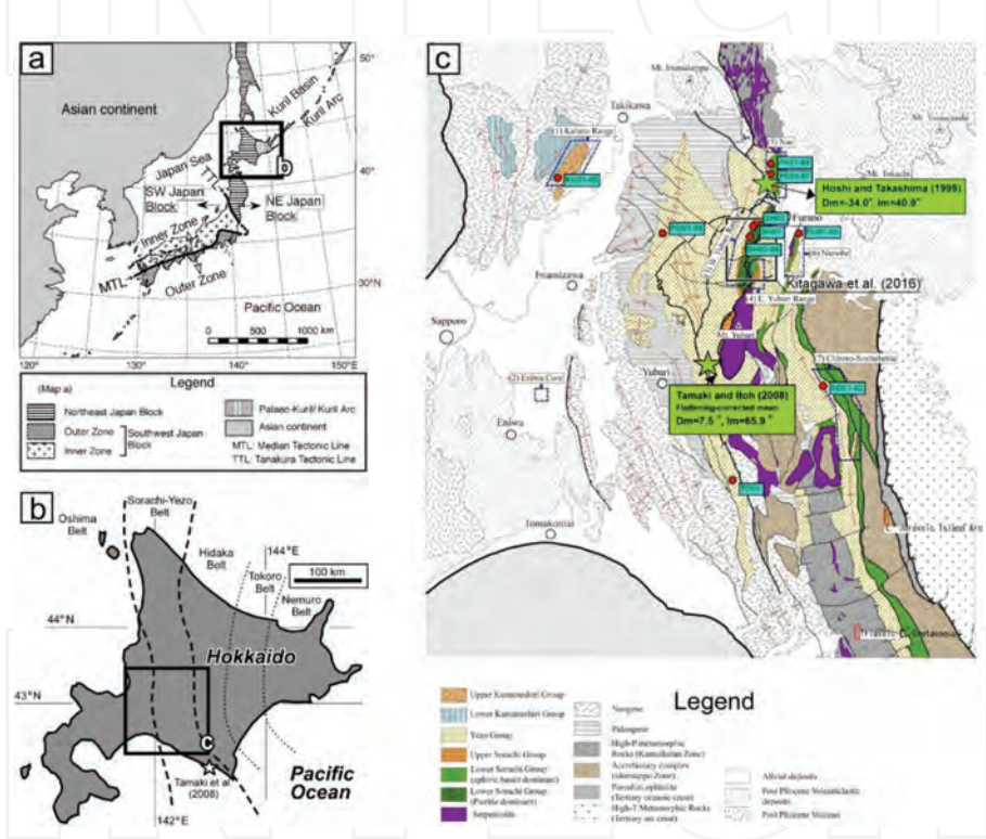
Figure 1. Index maps of study area. (a) Regional configuration and constituents of the Japanese Islands. (b) Pre-Cenozoic tectonic divisions in Hokkaido. (c) Geologic units around the sampling areas. Paleomagnetic sampling points are shown by dots. Stars and an enclosure indicate areas of previous paleomagnetic studies [4, 7, 10, 11].
