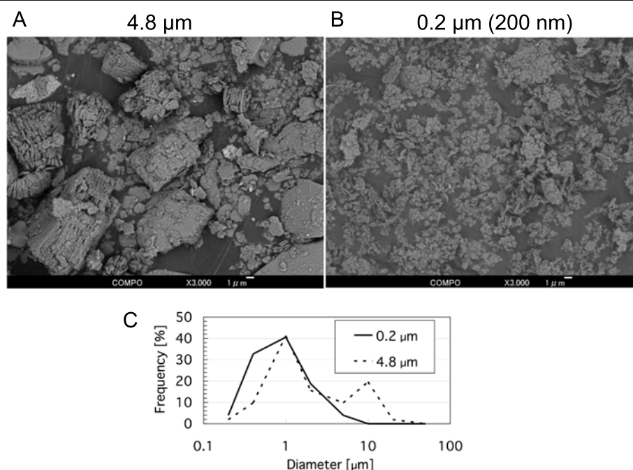
Fig. 1 SEM images of kaolin micro- and nano-particles. The reflected electron images of micro-particles ( a ; 4.8 \mu\text{m} ) and nano-particles ( b ; 0.2 \mu\text{m} ) were obtained at E = 5 \text{ kV} , \times 3000 . Scale bar indicates 1 \mu\text{m} . c : The size distributions of the particles
