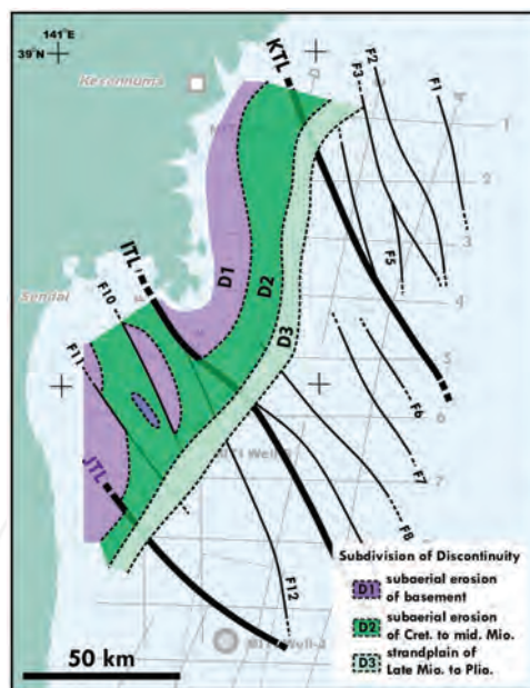
Figure 6. Map showing the distribution of discontinuity and its subdivisional zones.
