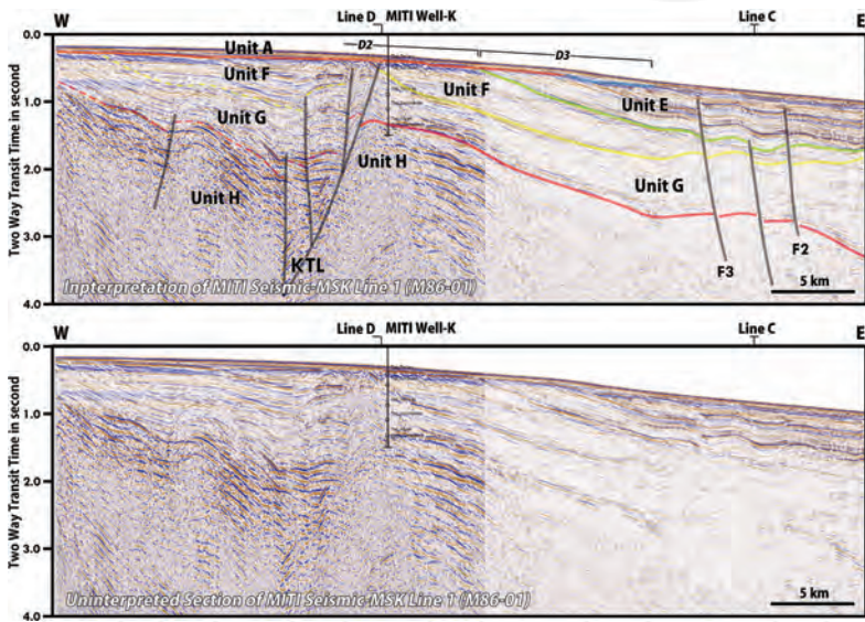
Figure 3. Uninterpreted section of MITI Seismic-MSK Line 1 (below), and its structural and stratigraphic interpretation (above).
