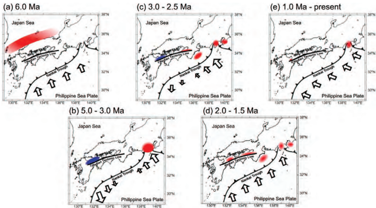
Figure 14. Spatiotempora distribution of stress-strain regimes in southwest Japan, the southern Japan Sea shelf, and a kinematic model of the Philippine Sea/Eurasian plate convergence since 6 Ma (a to e) compiled from [17, 18]. The red and blue areas represent areas of compressive (contractional) and tensile (extensional) stress (strain), respectively. Modes of the Philippine Sea Plate convergence are shown schematically by the length and azimuth of the arrows.
