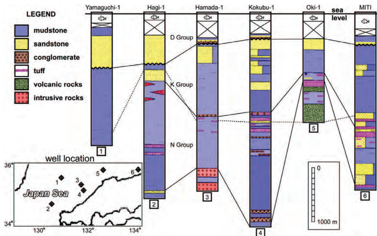
Figure 11. Stratigraphy of the offshore boreholes described by [5, 8]. Their localities are also shown in Figure 2. The solid and broken lines indicate unit boundaries and the 0.6% Ro (vitrinite reflectance) contour, respectively.
