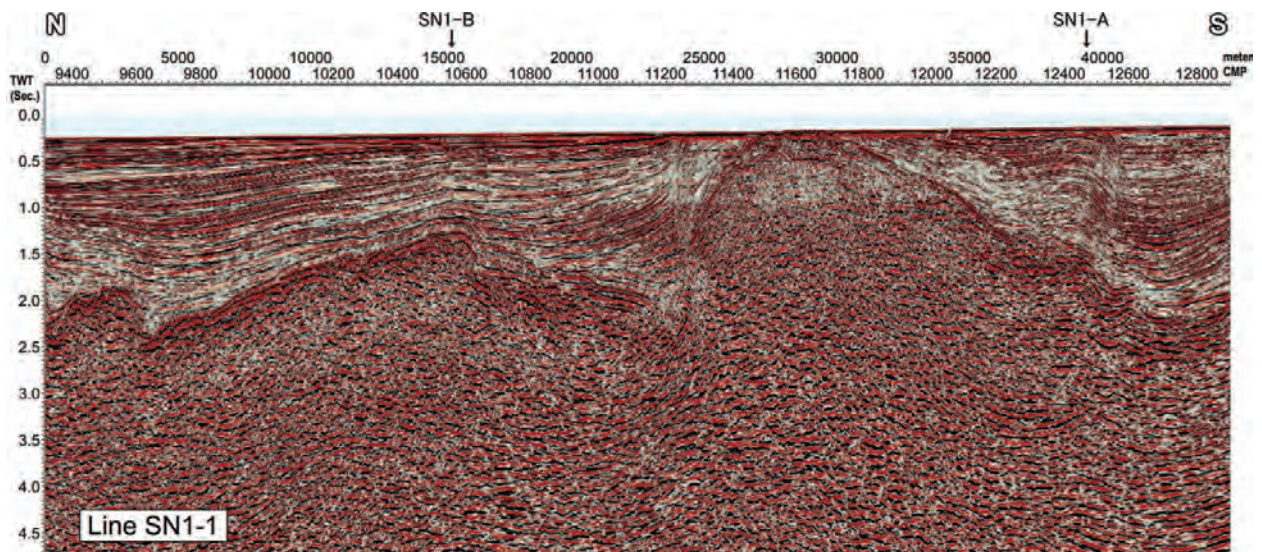
Figure 3. Reflection seismic profile (time migration; SN1-1) on the southwestern shelf of the Japan Sea. See Figure 2 for line locations.
