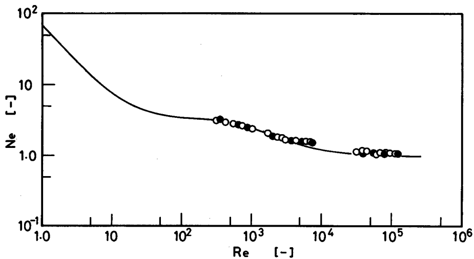
Fig. 5 Power correlation of 50^\circ -obliquely corrugated tank with liquid single phase for different impeller clearance: \circ C = H/2 ; \bullet C = H/3 — Rushton et al. 6)
